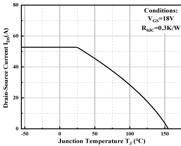
Maximum I_{DS} vs. Case Temperature
