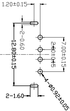
FRONT EDGE OF CONNECTOR PCB LAYOUT (T=1.60mm)
