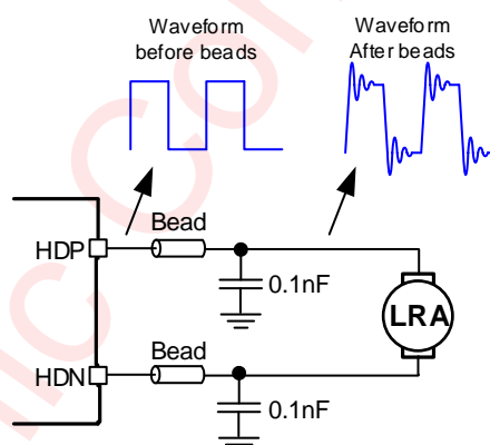
Figure 20 Ferrite Chip Bead and capacitor
