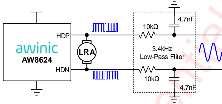
Figure 6 AW8624 test setup
