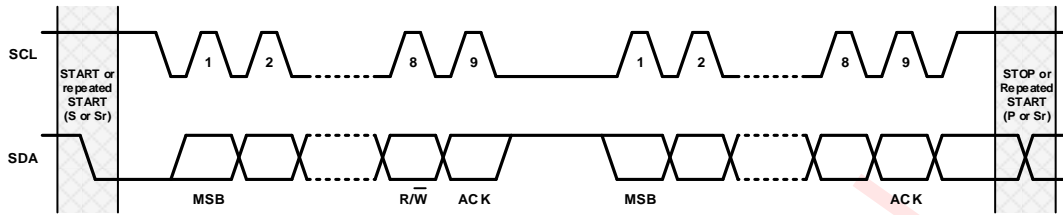
Figure 17 Data transmission on the I 2 C bus
