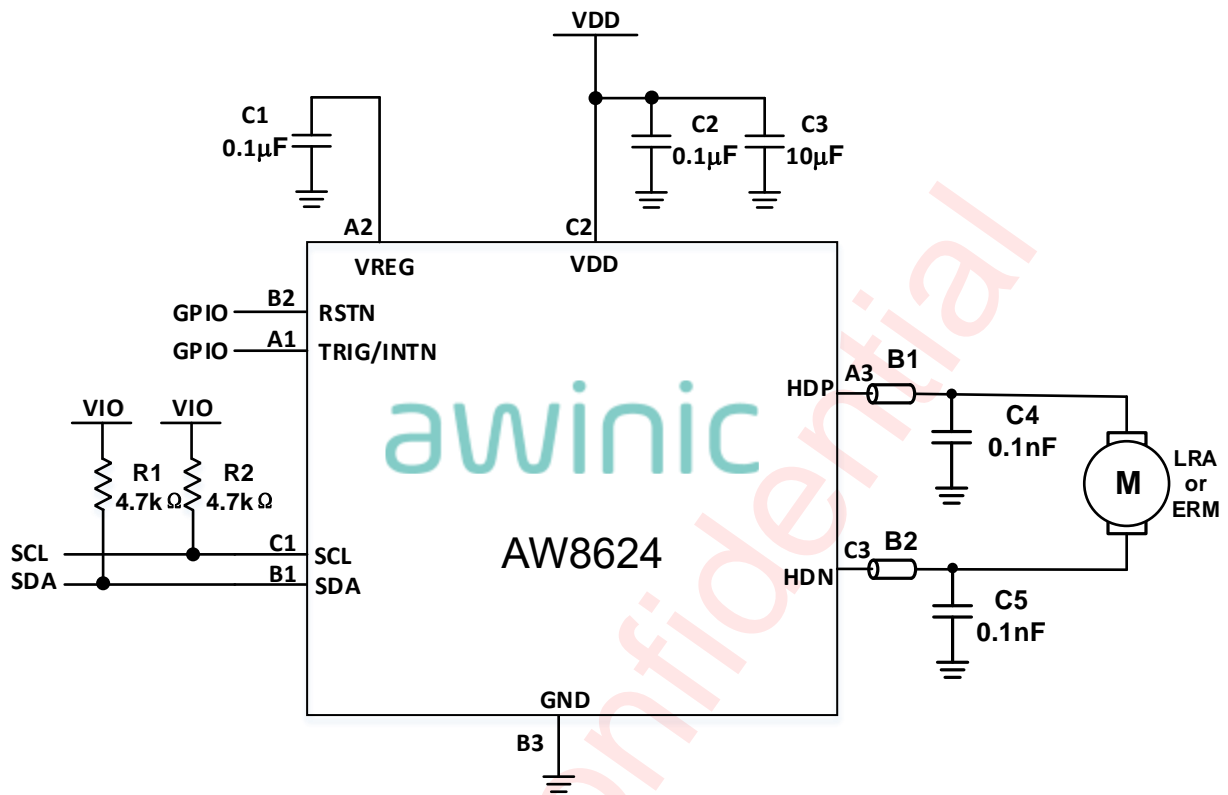
Figure 1 Typical Application Circuit of AW8624
