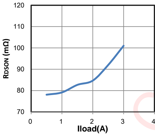
Figure 14 R_{DS(on)} vs. I_{load}
