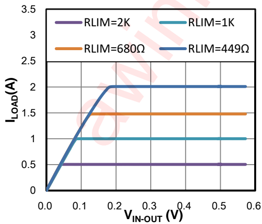
Figure 16 I_{LOAD} vs. V_{IN-OUT}
