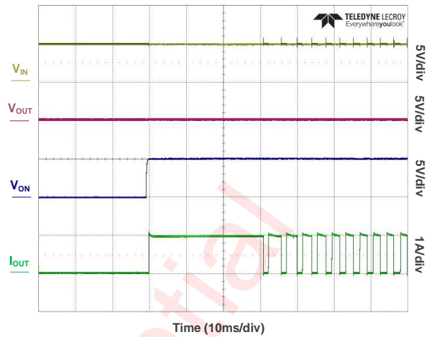
Figure 25 Starting up into shorted output
