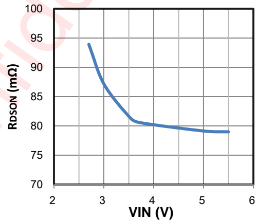
Figure 15 R_{DS(on)} vs. V_{IN}
