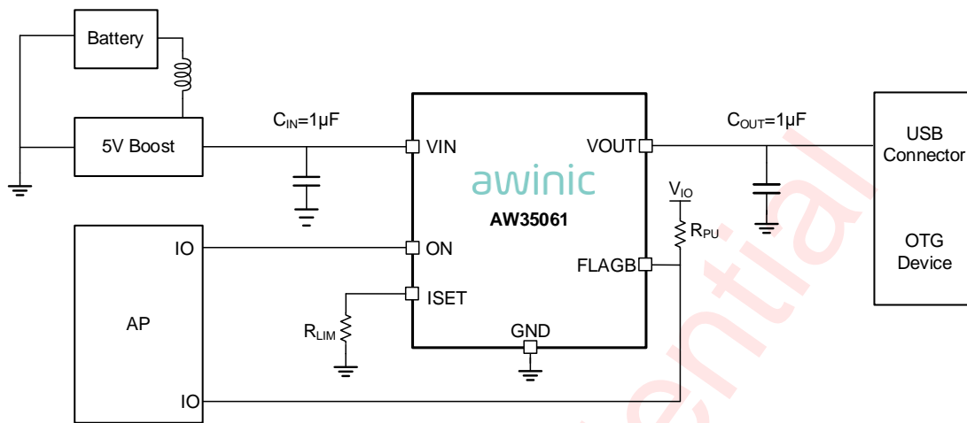
Figure 4 AW35061 Application circuit
