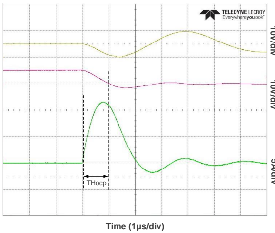
Figure 24 THocp Response Time
