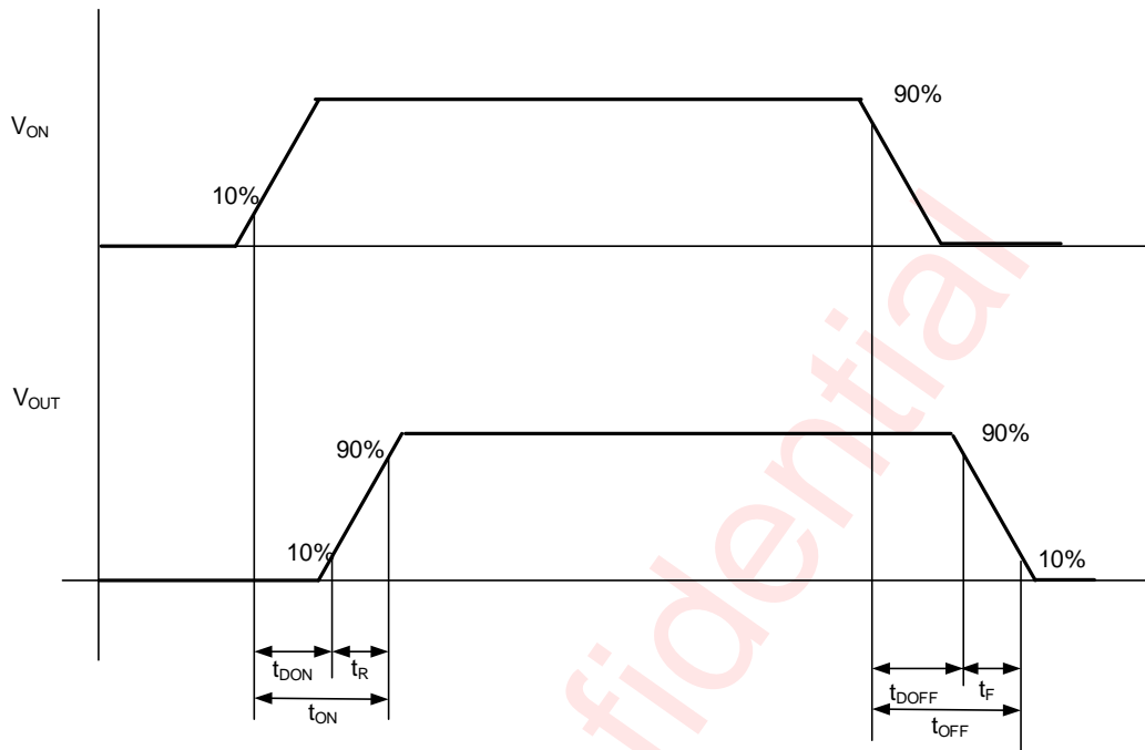
Figure 5 AW35061 Timing Diagrams
