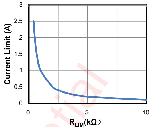
Figure 13 Current Limit Threshold vs. R_{LIM}
