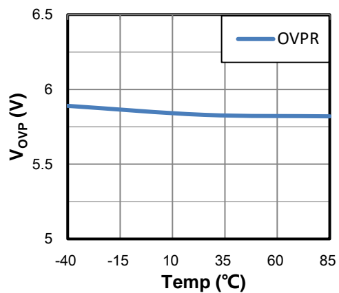
Figure 11 OVP Threshold Voltage vs. Temperature
