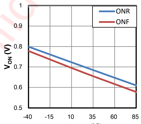
Figure 9 ON Threshold Voltage vs. Temperature
