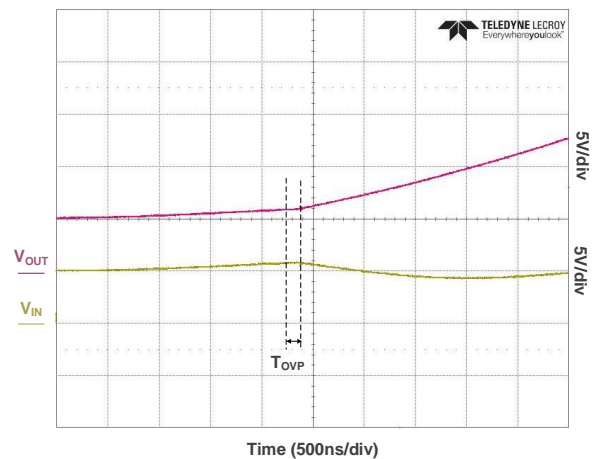
Figure 17 Over Voltage Protection
