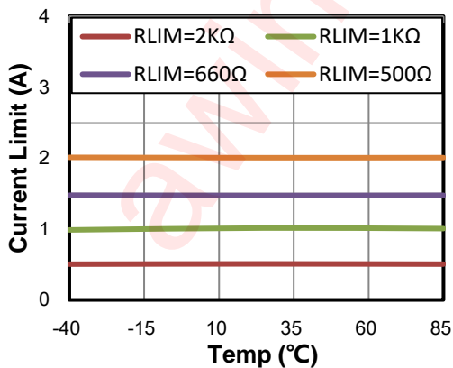
Figure 10 Current Limit Threshold vs. Temperature
