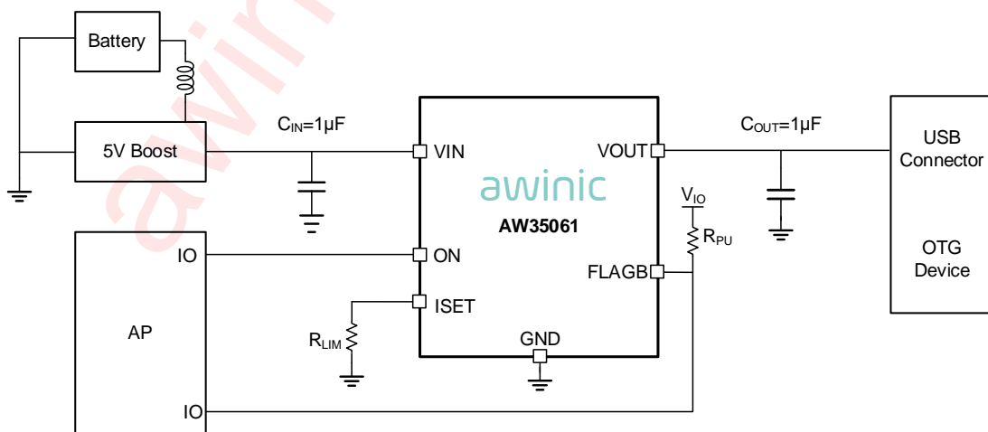
Figure 1 Typical Application Circuit of AW35061
