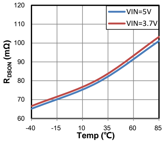
Figure 12 R_{DS(on)} vs. Temperature
