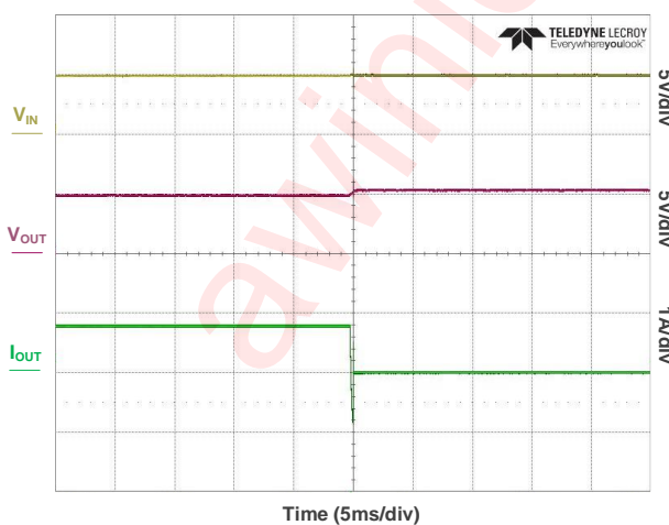
Figure 28 Reverse Current Blocking
