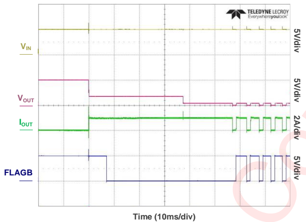
Figure 26 Output Short Circuit Protection
