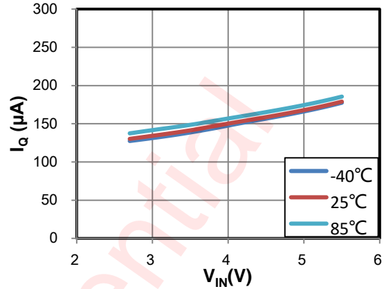
Figure 7 Quiescent Current vs. V_{IN}
