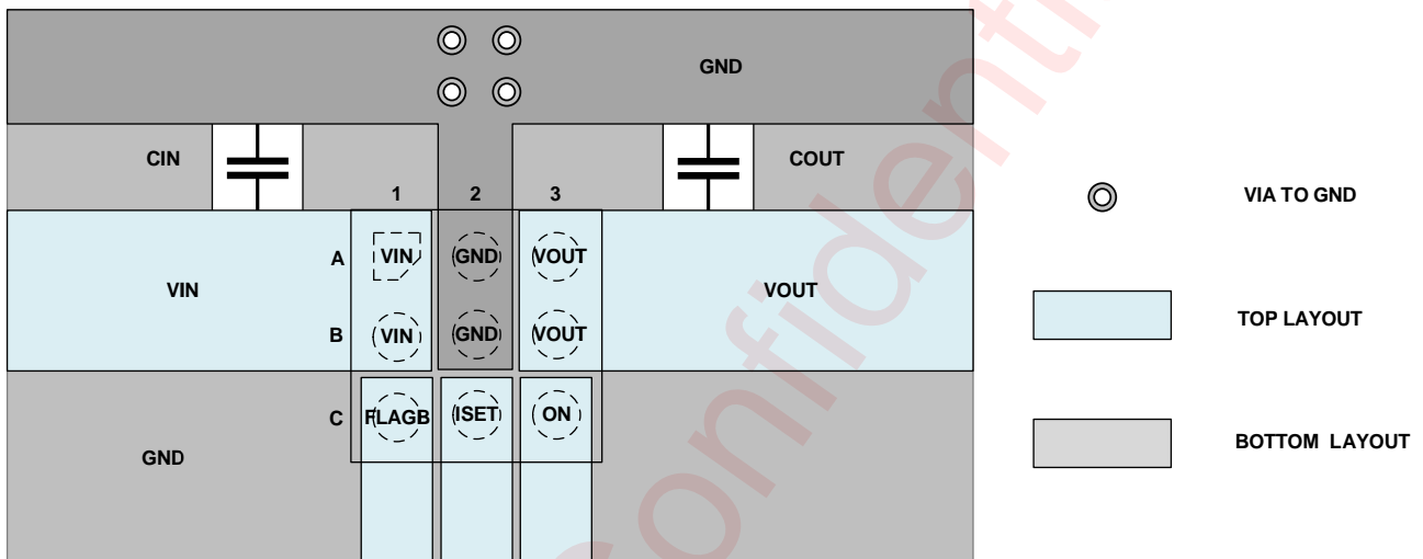
Figure 31 AW35061 PCB Layout Example
