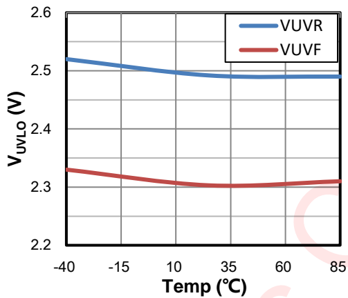
Figure 8 UVLO Threshold Voltage vs. Temperature
