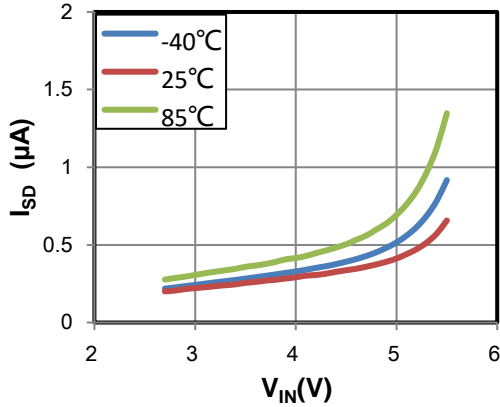
Figure 6 Shutdown Current vs. V_{IN}
