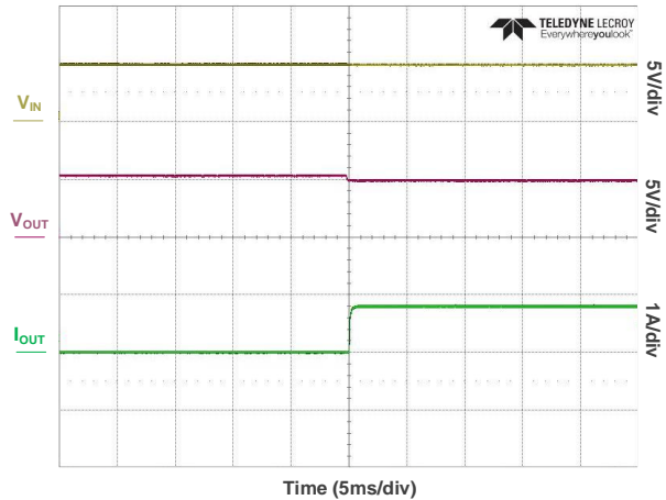
Figure 29 Recovery from Reverse Current Blocking
