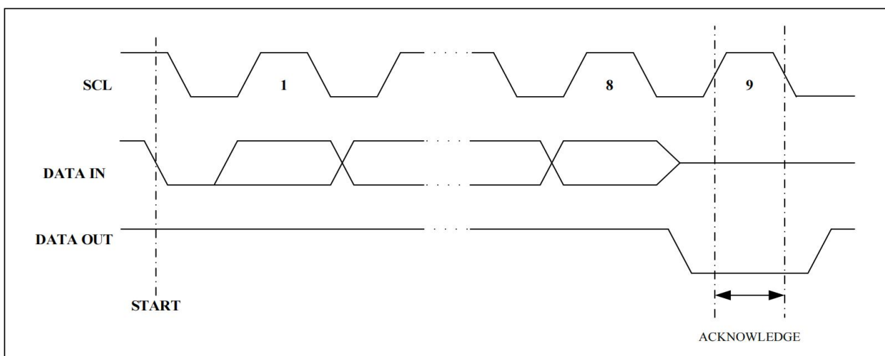
Figure 4. Output Acknowledge
