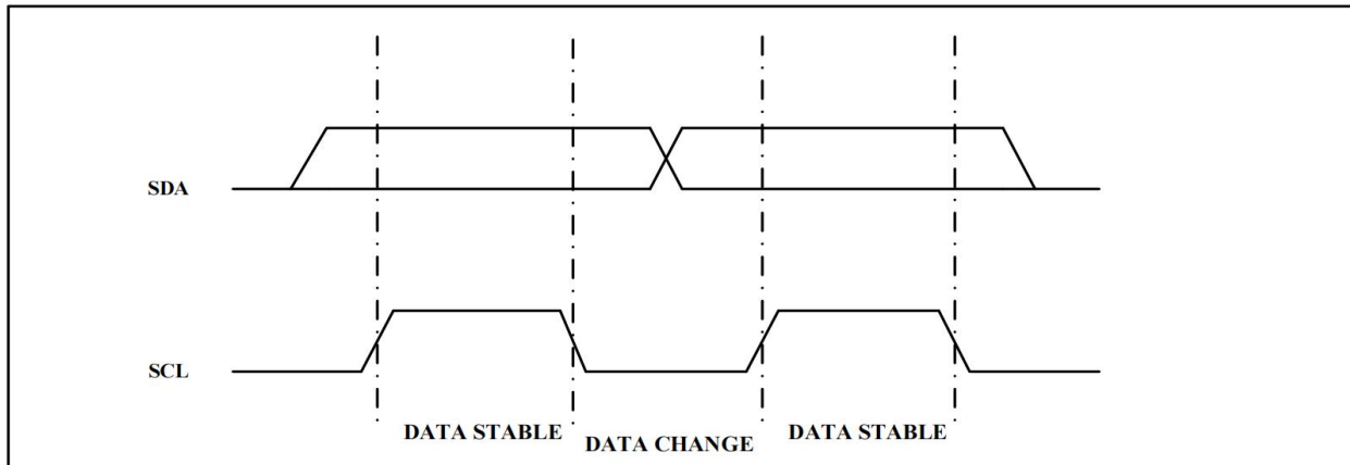
Figure 2. Data Validity
