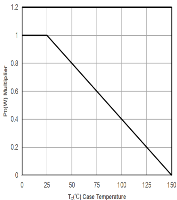
Power Dissipation P_{tot}=f(T_C)
