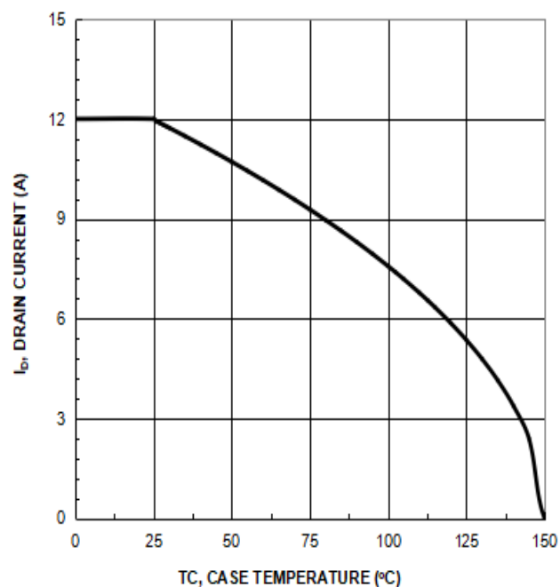
Maximum Drain Current I_D=f(T_C)
