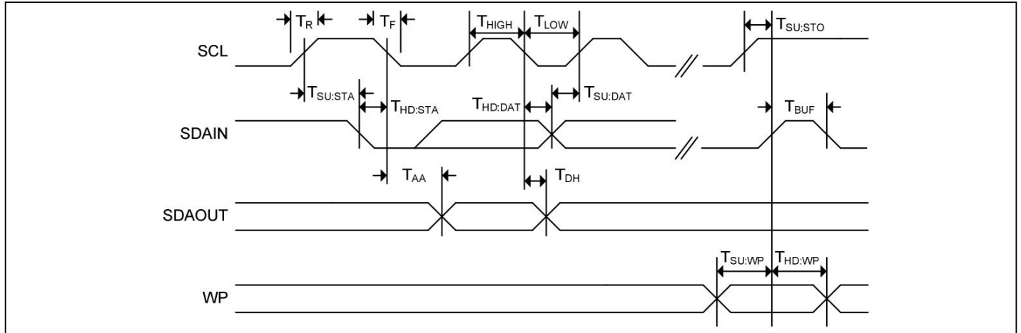
Figure 1-11. Bus Timing
