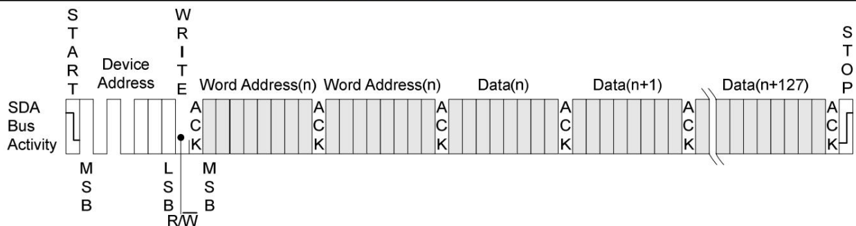
Figure 1-7. Page Write
