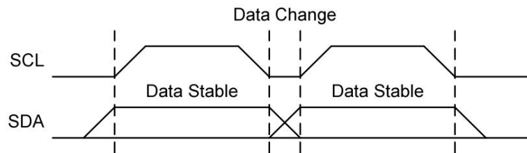
Figure 1-4. Data Validity Protocol
