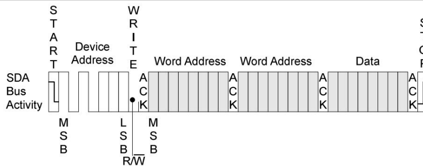
Figure 1-6. Byte Write
