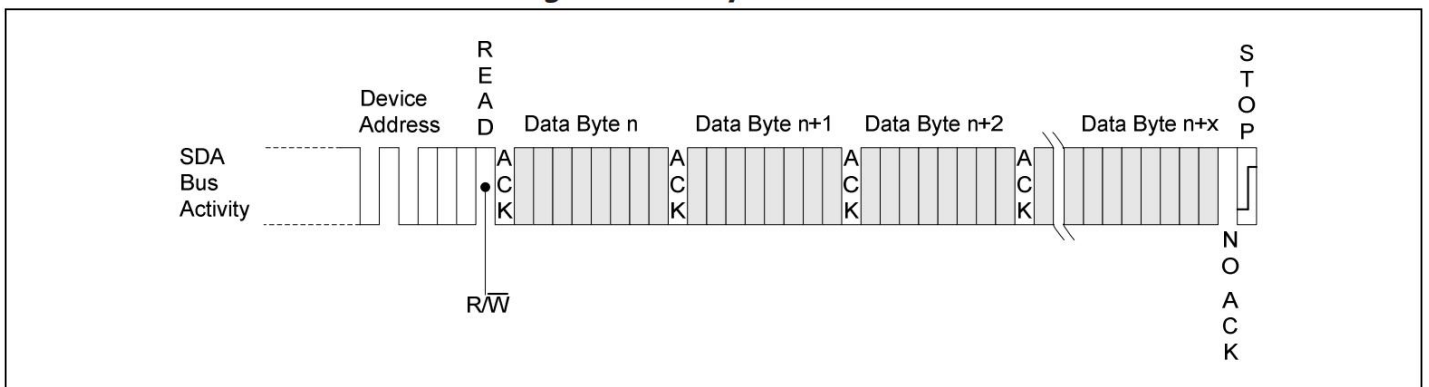
Figure 1-10. Sequential Read
