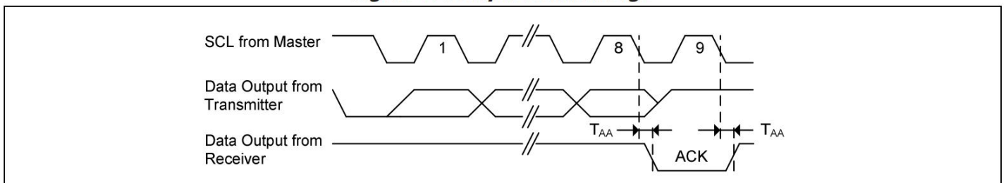
Figure 1-2. output Acknowledge
