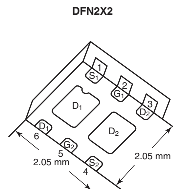
DFN2X2
