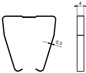
18FF-H1(金属卡簧)
