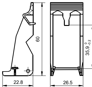
18FF-H4 (塑料卡簧)
