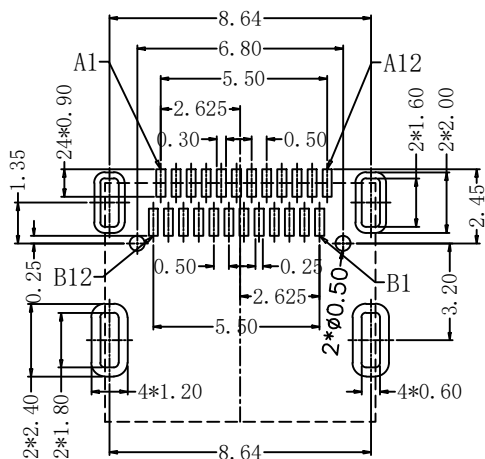
RECOMMENDED PCB LAYOUT, TOP VIEW (TICHNESS=1.0~1.2MM; TOLERANCE:±0.05)
