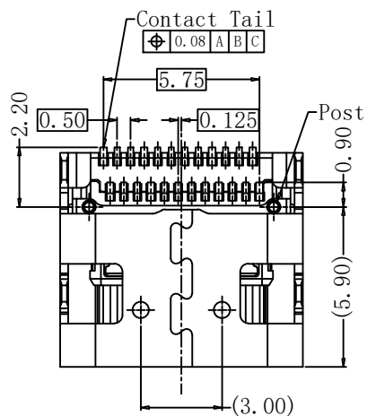
RECOMMENDED PCB LAYOUT, TOP VIEW (TICHNESS=1.0~1.2MM; TOLERANCE:±0.05)
