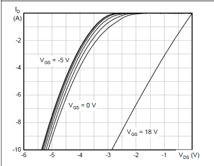
Figure 13. Body Diode Characteristics, T_J = 25^\circ\text{C}
