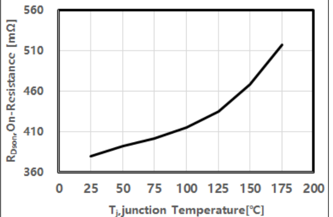
Figure 12. On-Resistance vs. Temperature
