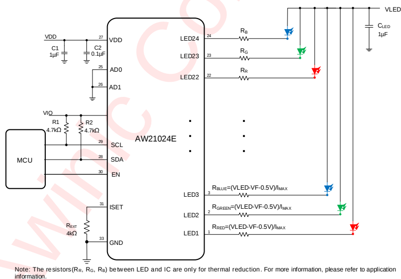
Figure 4 AW21024E Application Circuit
