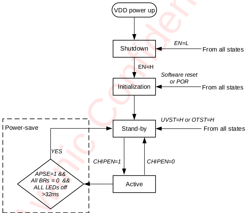
Figure 8 AW21024E Operating Mode Transition
