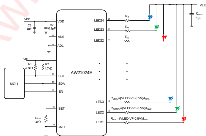
Figure 1 AW21024E Application Circuit
