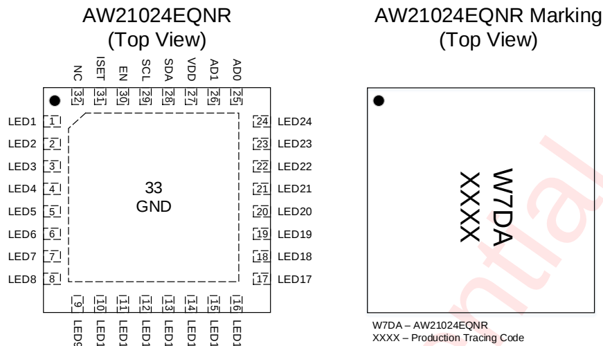
Figure 2 Pin Configuration and Marking
