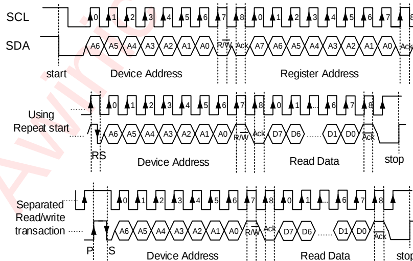
Figure 13 I 2 C Read Byte Cycle
