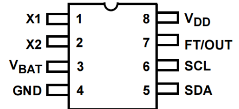
ISL12008
