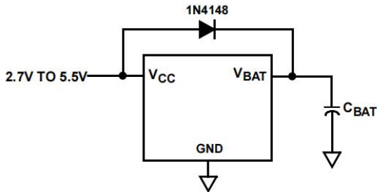
FIGURE 18. SUPERCAPACITOR CHARGING CIRCUIT
