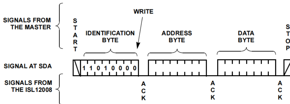
FIGURE 12. BYTE WRITE SEQUENCE
