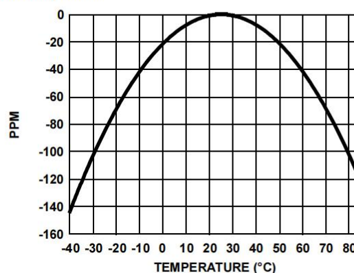
FIGURE 15. RTC CRYSTAL TEMPERATURE DRIFT
