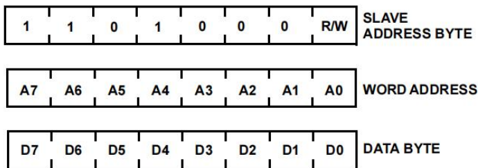
FIGURE 13. SLAVE ADDRESS, WORD ADDRESS, AND DATA BYTES
