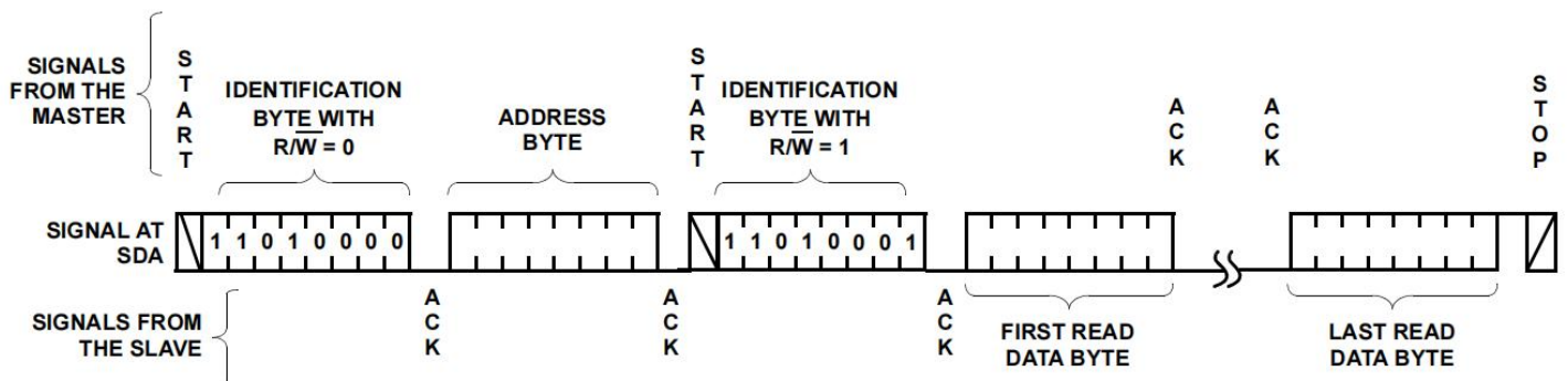
FIGURE 14. READ SEQUENCE
