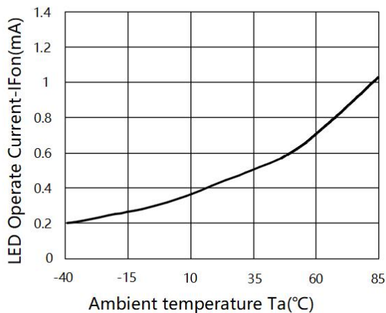
Fig.5 LED Operate Current-IFon(mA) vs Ambient Temperature
