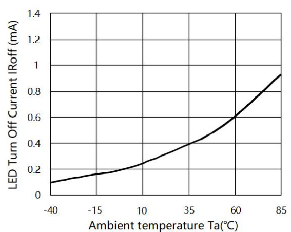
Fig.6 LED Turn Off Current-IRoff(mA) vs Ambient Temperature
