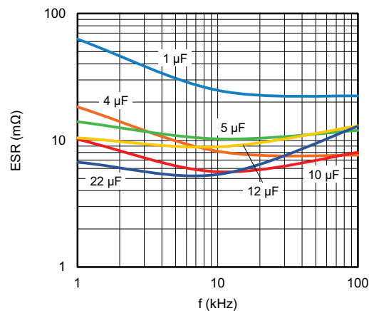
ESR as function of frequency (1200 V_{DC} ) (typical curve)
