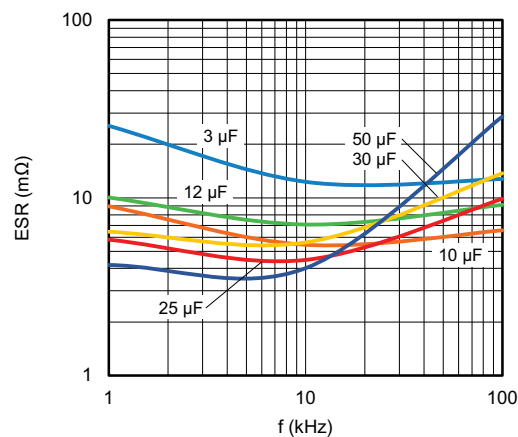
ESR as function of frequency (800 V_{DC} ) (typical curve)
