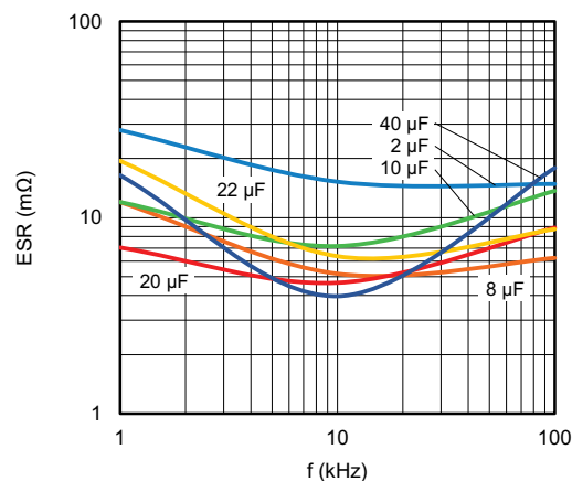
ESR as function of frequency (920 V_{DC} ) (typical curve)
