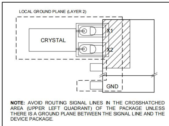
Figure 2. Recommended Layout for Crystal
