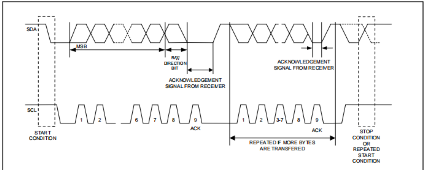
Figure 3. Data Transfer on I 2 C Serial Bus
