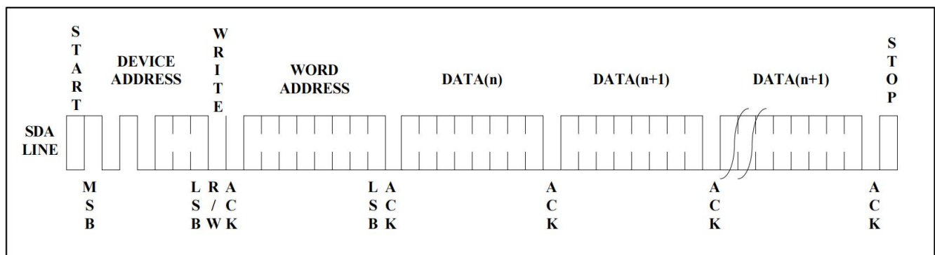
Figure 7. Page Write
