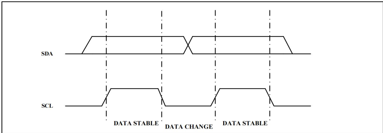
Figure 2. Data Validity
