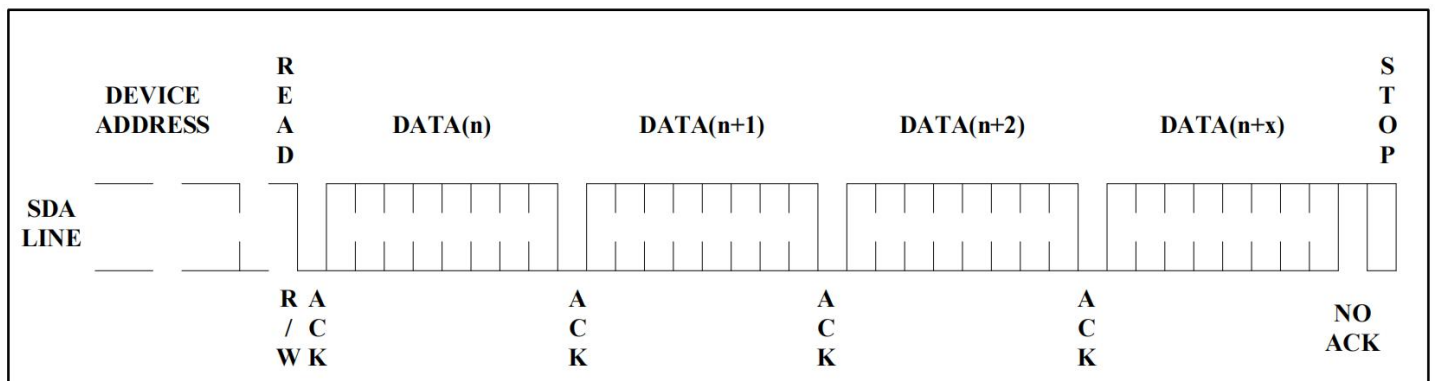
Figure 10. Sequential Read
