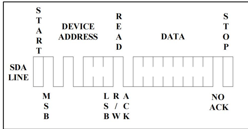
Figure 9. Random Read
