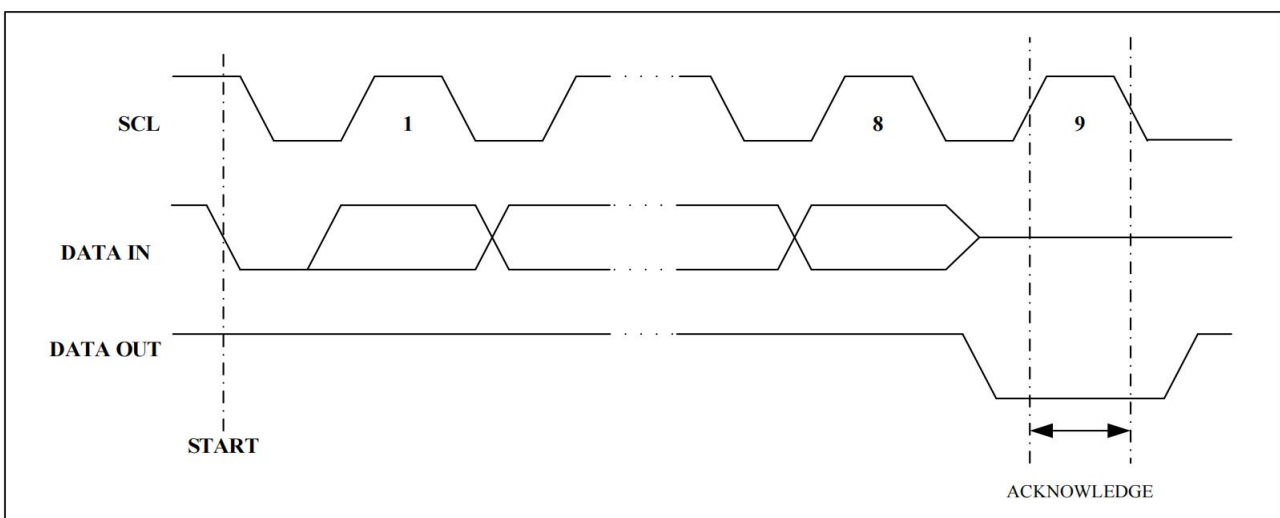
Figure 4. Output Acknowledge
