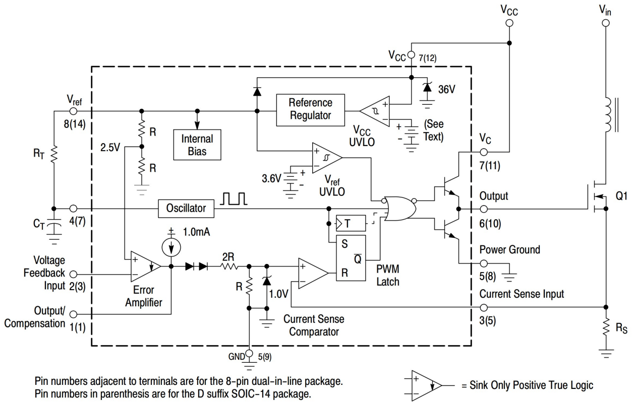
Figure 16. Representative Block Diagram
