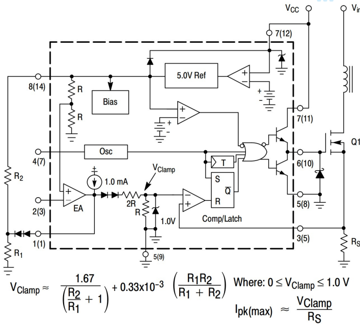
Figure 20. Adjustable Reduction of Clamp Level
