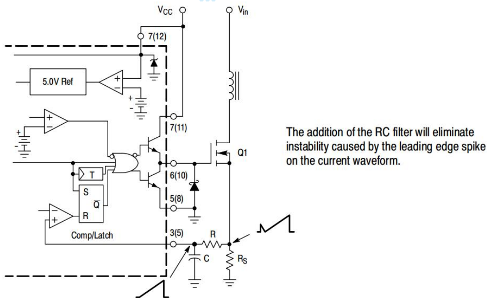
Figure 24. Current Waveform Spike Suppression
