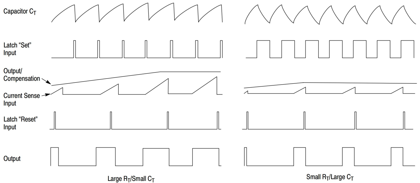
Figure 17. Timing Diagram
