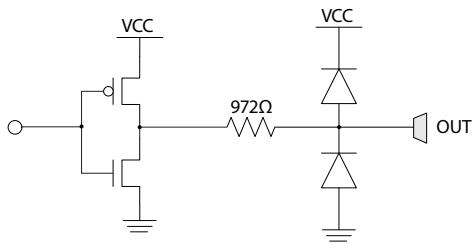
Figure 3-3: Low-speed Outputs (LOCKED, LOS, \overline{\text{SD/H\overline{D}}} )
