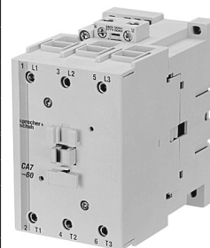
CA7-60D Contactor
