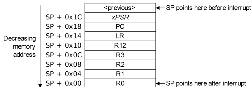
Figure 26-10. Exception Entry Stack Contents
