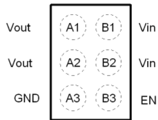
Laser Mark View
