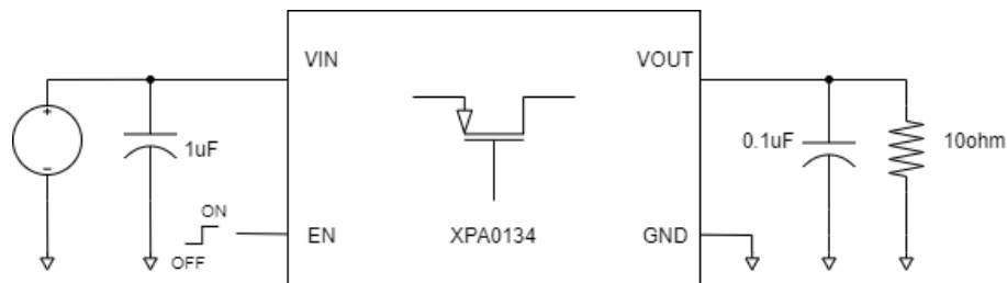
Test circuit
