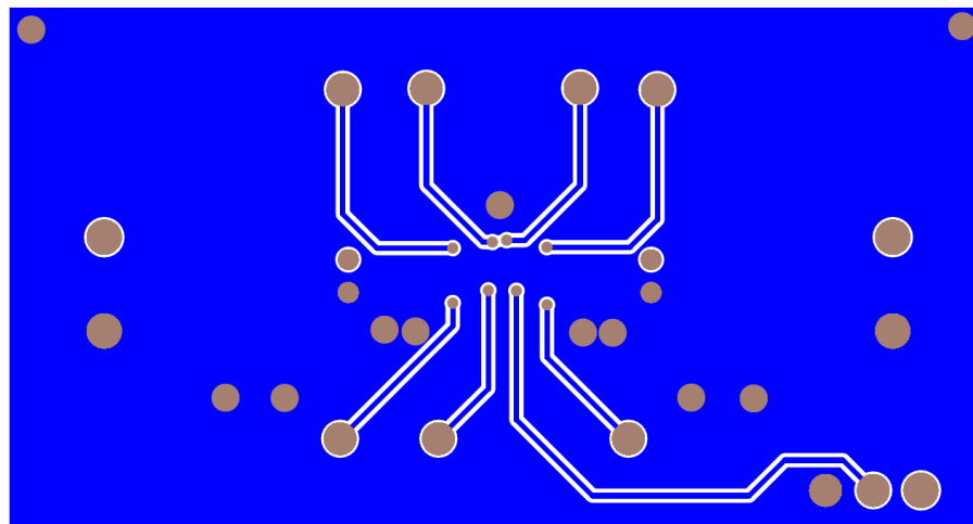
Demo board PCB Bottom View
