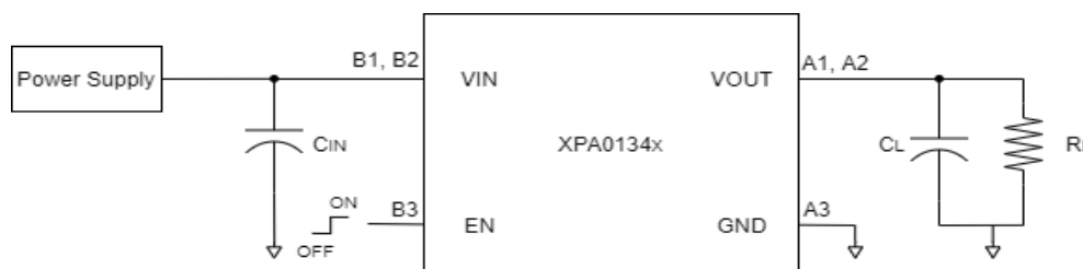
Typical Application Circuit
