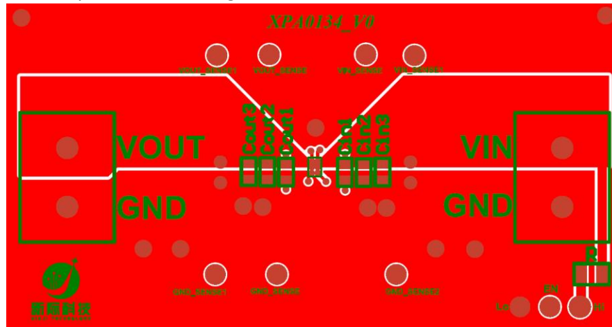
Demo board PCB Top View
