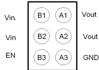
Bump View
