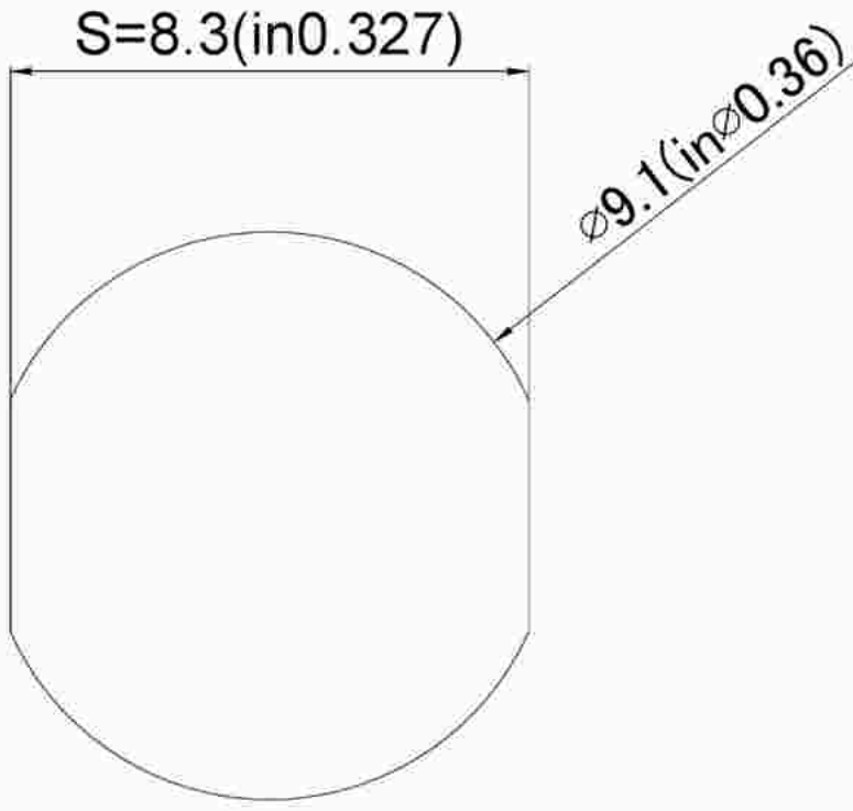
Pane hole size (面板开孔尺寸)
