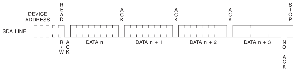
Figure 12. Sequential Read
