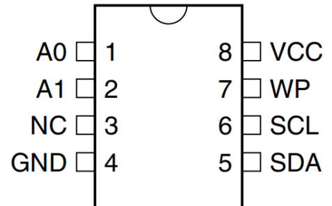
8-lead PDIP
