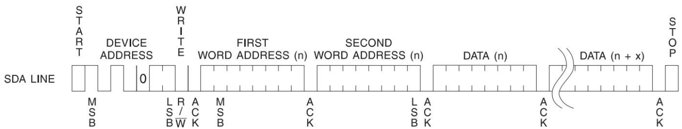
Figure 9. Page Write
