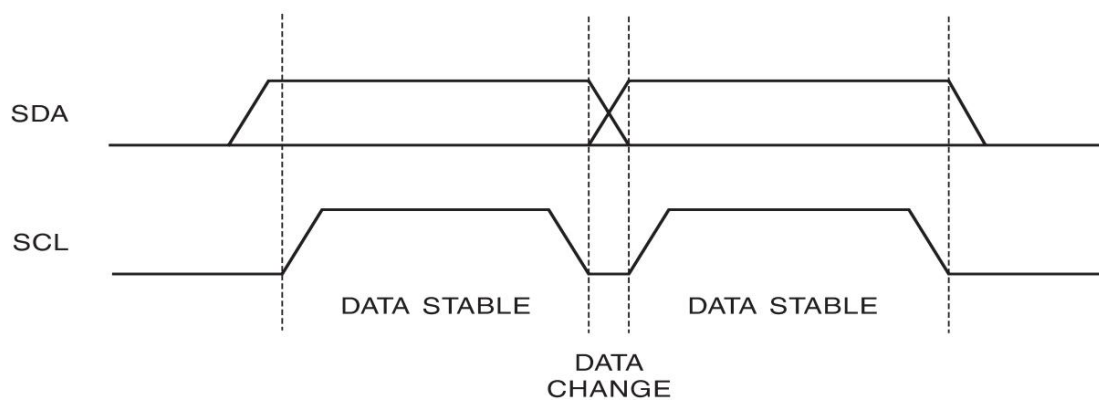
Figure 4. Data Validity
