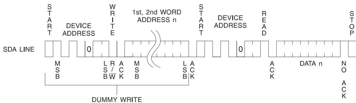
Figure 11. Random Read
