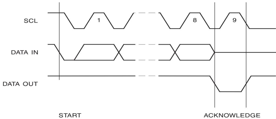
Figure 6. Output Acknowledge
