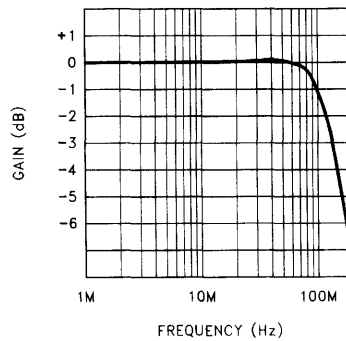
EL2140 V_{REF} Frequency Response
