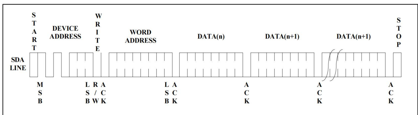
Figure 7. Page Write
