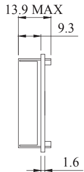
LED B/L
