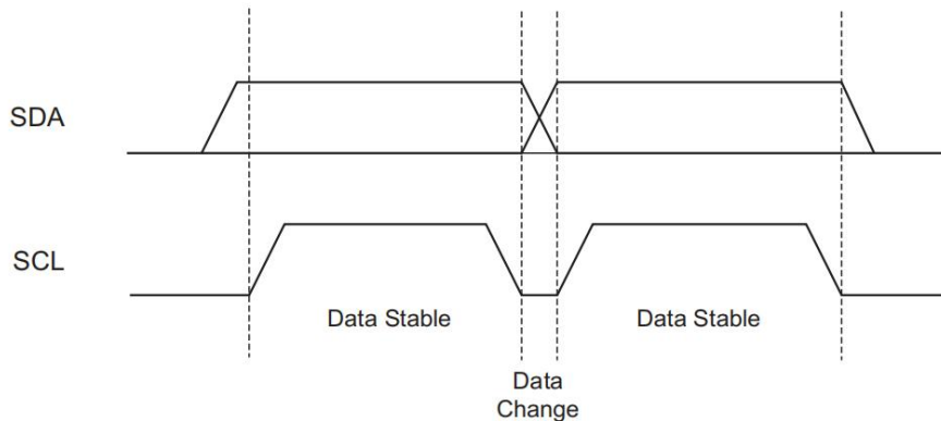
Figure 6-1. Data Validity
