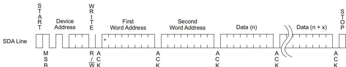
Figure 8-2. Page Write
