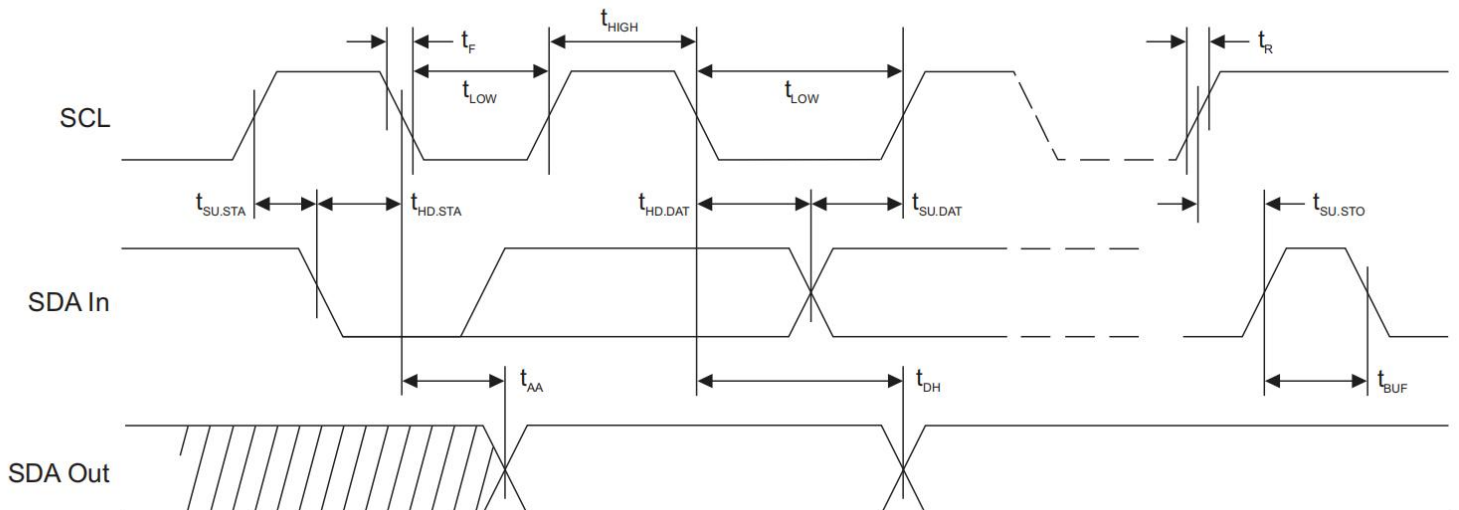
Figure 6-4. Bus Timing
