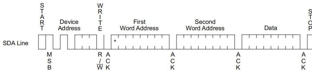
Figure 8-1. Byte Write
