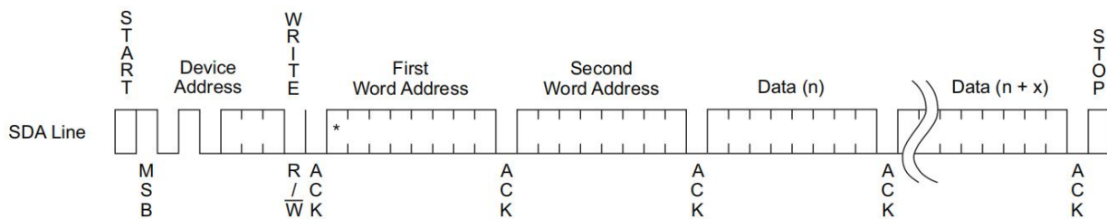
Figure 8-2. Page Write
