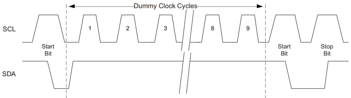
Figure 6-3. Software Reset
