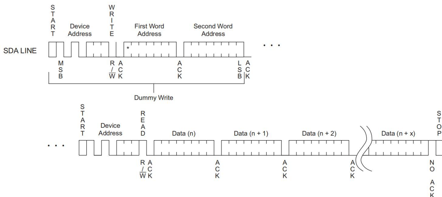
Figure 9-3. Sequential Read
