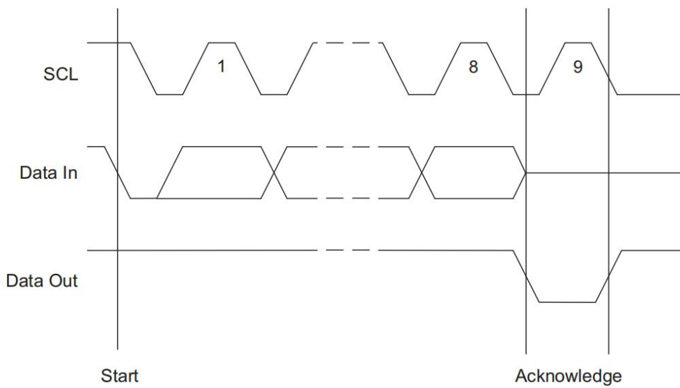
Figure 6-6. Output Acknowledge
