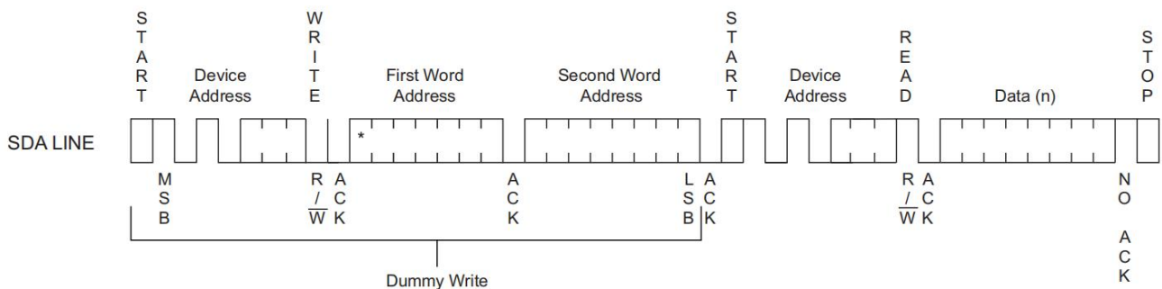
Figure 9-2. Random Read
