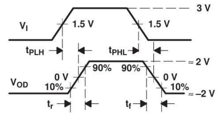
Figure 9. Driver Switching Test Circuit and Voltage Waveforms
