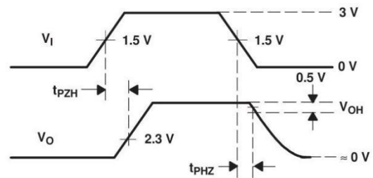
Figure 10. Driver High-Level Enable and Disable Time Test Circuit and Voltage Waveforms
