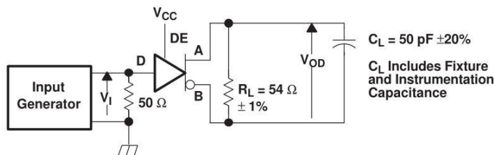
Figure 9. Driver Switching Test Circuit and Voltage Waveforms
