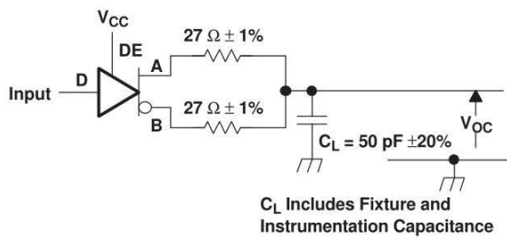
Figure 8. Test Circuit and Definitions for the Driver Common-Mode Output Voltage
