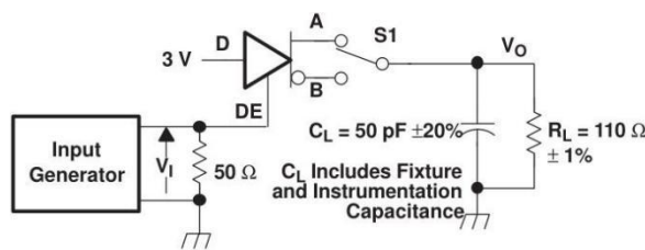
Figure 10. Driver High-Level Enable and Disable Time Test Circuit and Voltage Waveforms
