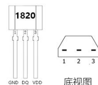
TO-92S (1820)
