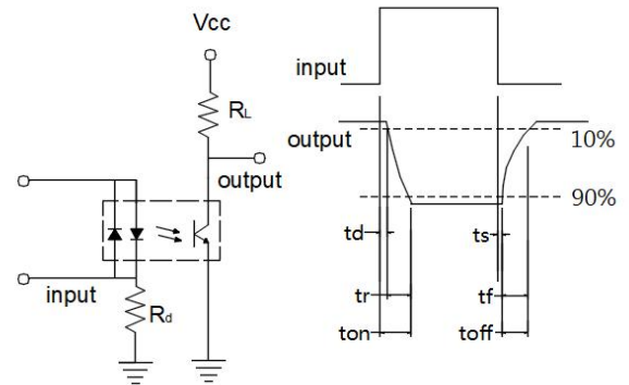
响应时间测试电路 Test Circuit for Response Time
