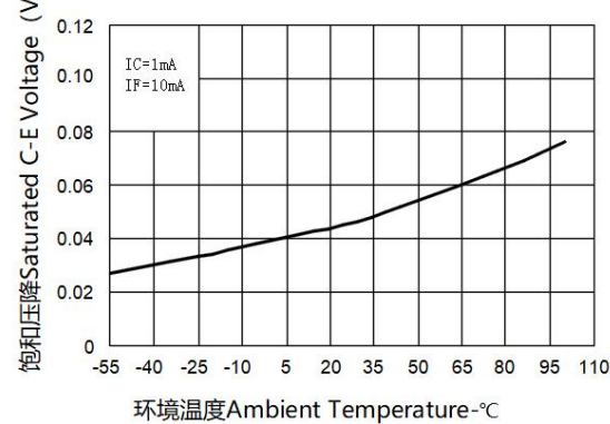
集电极-发射极饱和压降与环境温度特性曲线 Collector-emitter Saturation Voltage vs. Ambient Temperature
