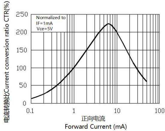
电流转换比与正向电流特性曲线 Relative Current Transfer Ratio vs. Forward Current
