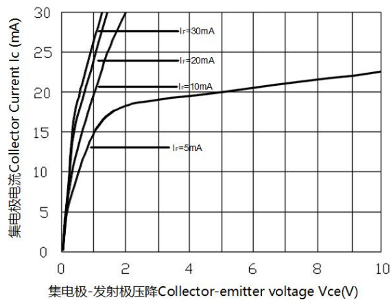
集电极电流与集电极-发射极电压特性曲线 Collector Current vs. Collect-emitter voltage
