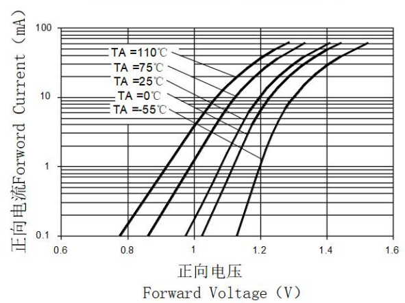
正向电流与正向压降特性曲线 Forward Current vs Forward Voltage
