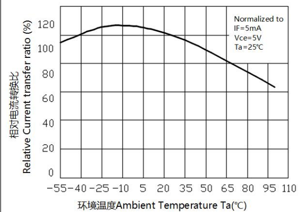
相对电流转换比与环境温度特性曲线 Relative Current Transfer Ratio vs. Ambient Temperature
