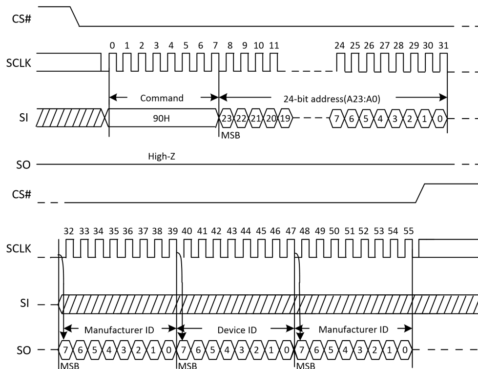
Figure 24. Read Manufacturer ID/ Device ID Sequence Diagram
