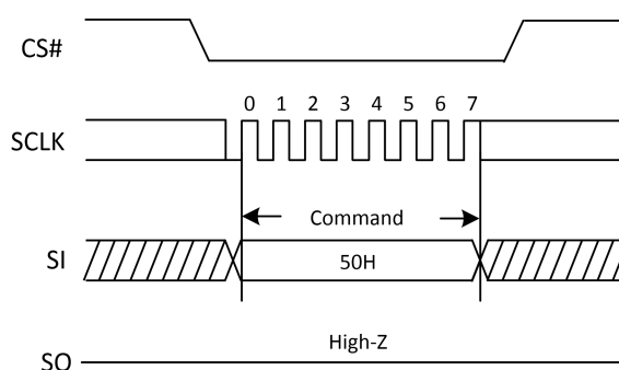
Figure 3. Write Enable for Volatile Status Register Sequence Diagram
