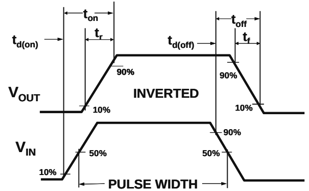
Figure 2: Switching Waveforms
