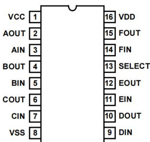
Figure 2.1 Top View
