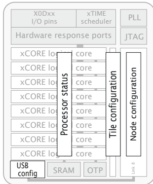
Figure 32: Registers
