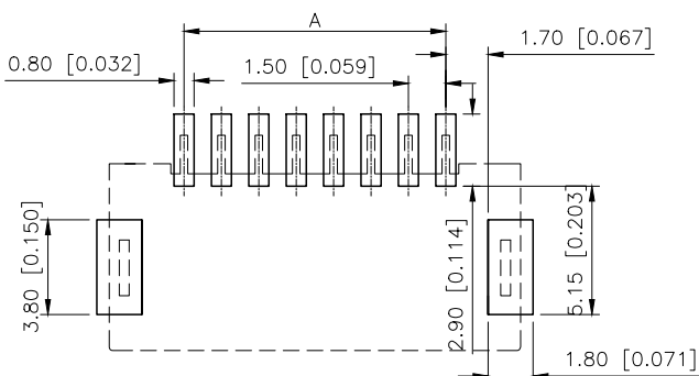
PCB LAYOUT(Tolerance:±0.05)
