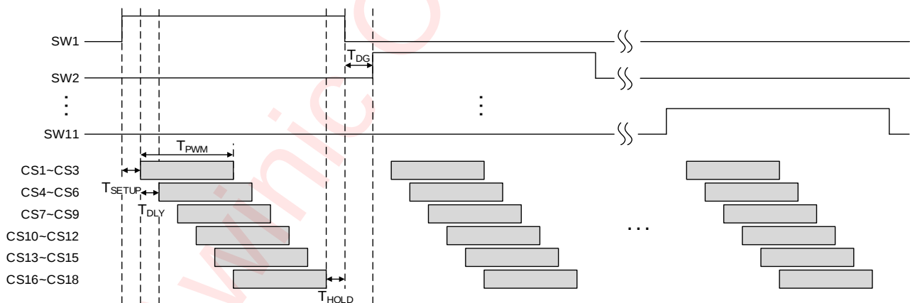
Figure 17 Scanning Timing
