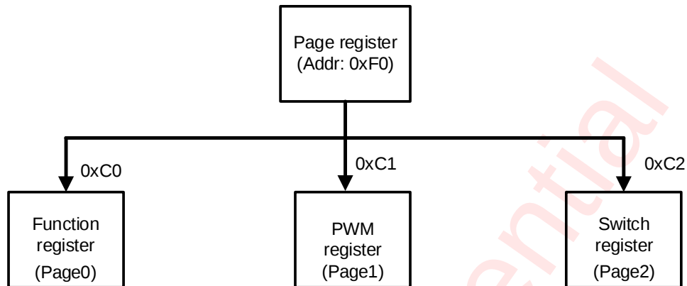
Figure 19 Register Control
