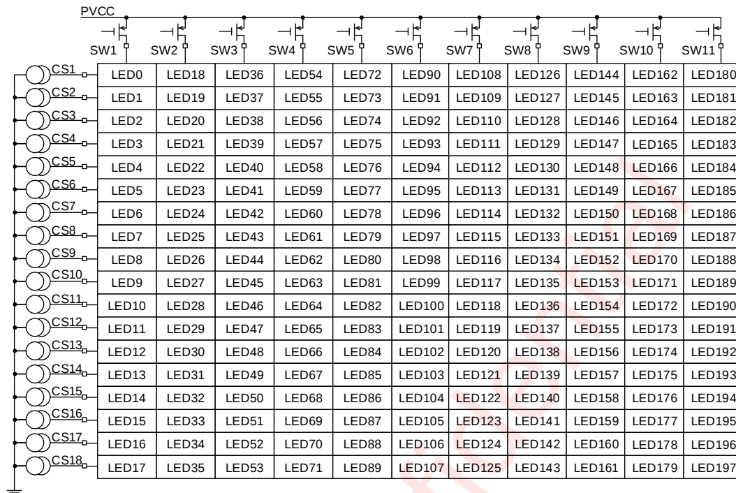
Figure 16 LED Location
