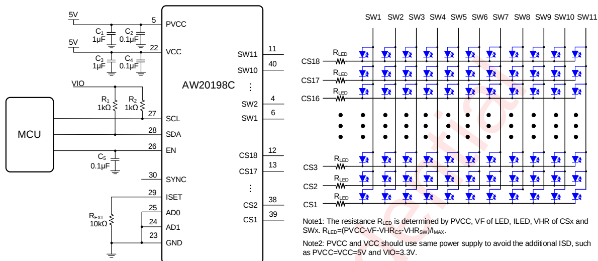
Figure 1 AW20198C Application Circuit
