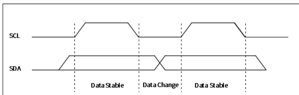
Figure 4-1 Data Validity
