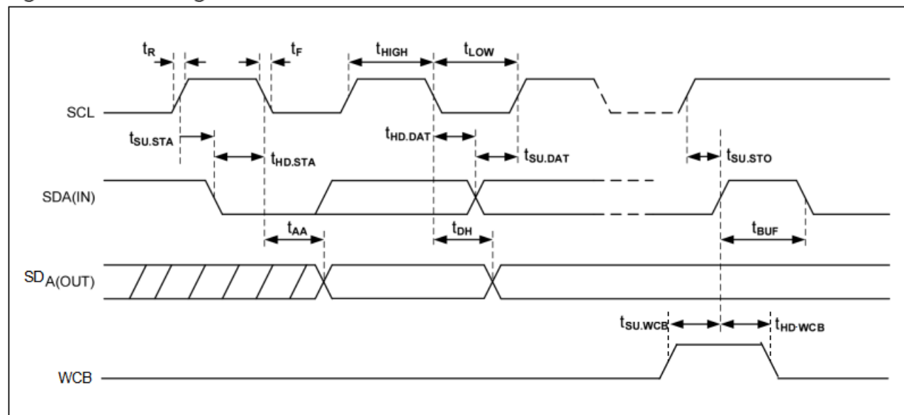
Figure 3-1 Bus Timing
