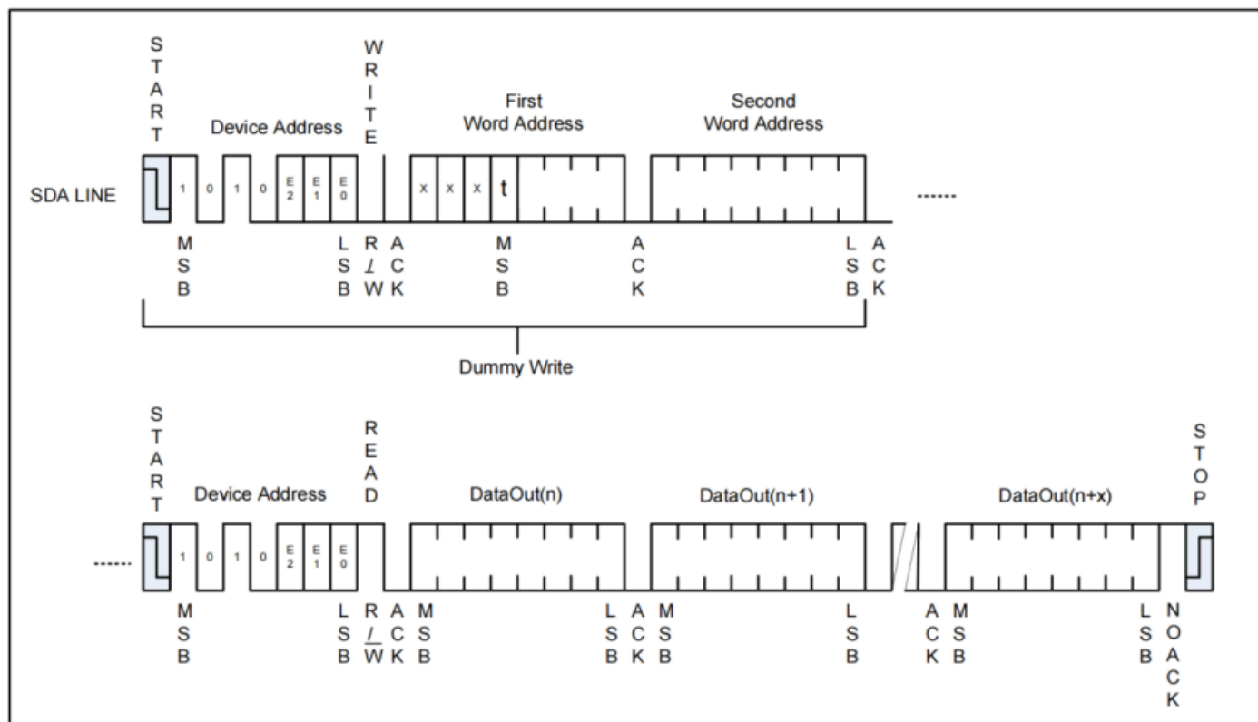
Figure 5-5 Sequential Read
