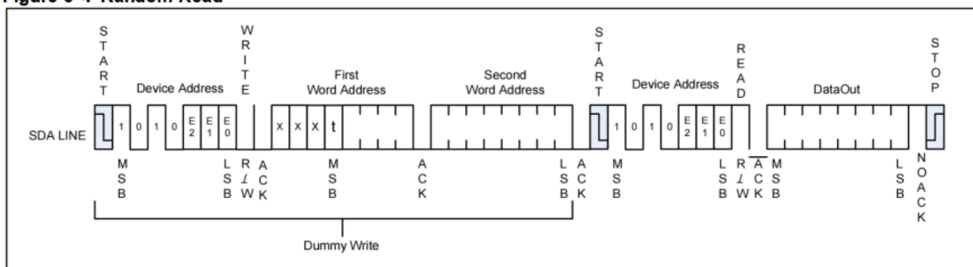
Figure 5-4 Random Read
