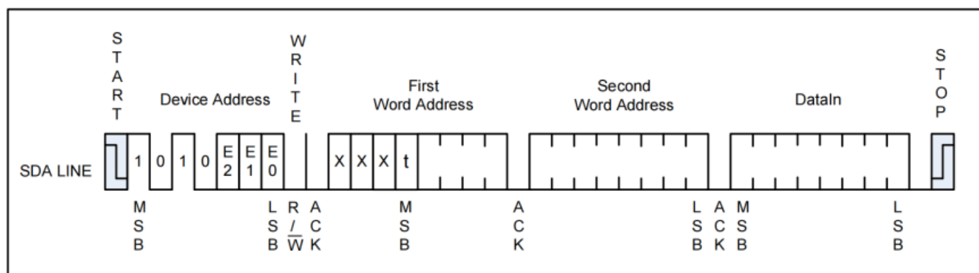
Figure 5-1 Byte Write
