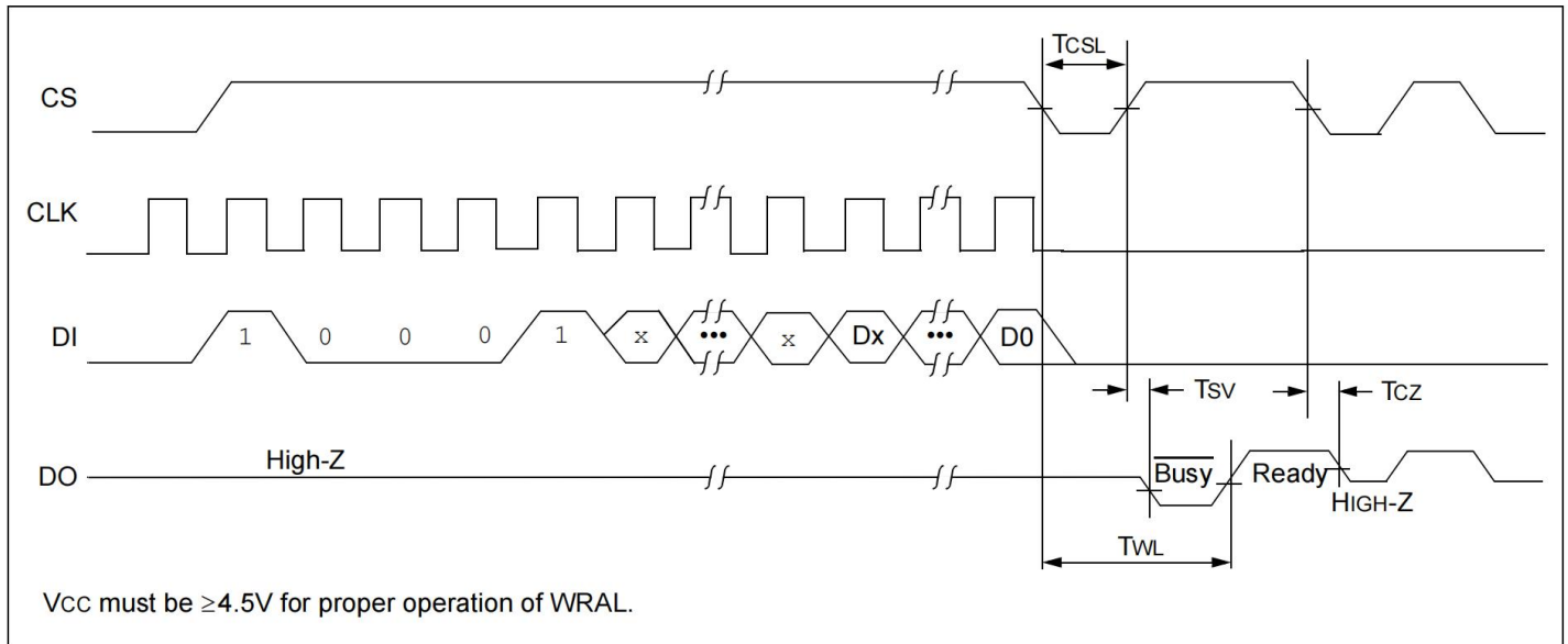
FIGURE 2-10: WRAL TIMING FOR 93AA AND 93LC DEVICES
