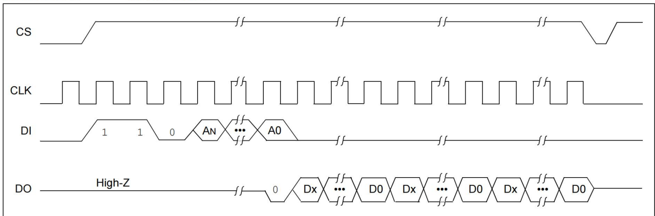
FIGURE 2-7: READ TIMING
