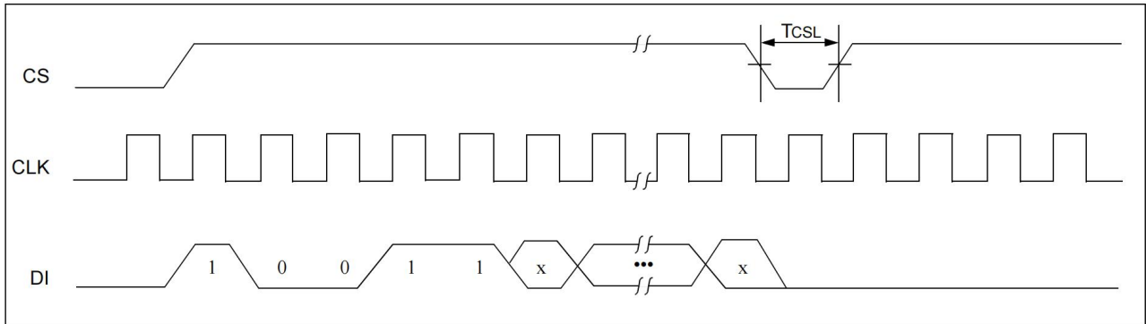
FIGURE 2-6: EWEN TIMING
