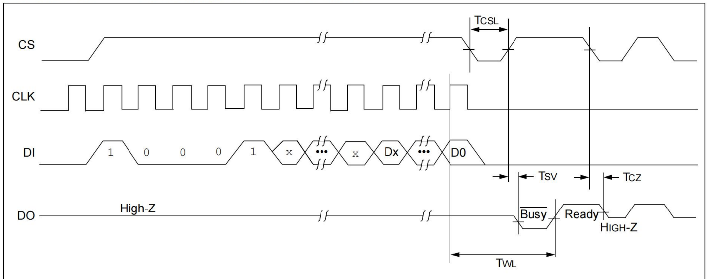
FIGURE 2-11: WRAL TIMING FOR 93C DEVICES
