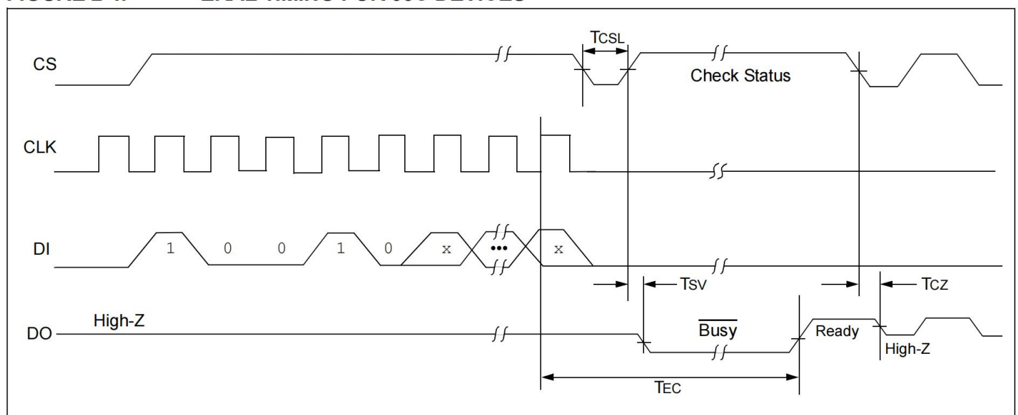
FIGURE 2-4: ERAL TIMING FOR 93C DEVICES
