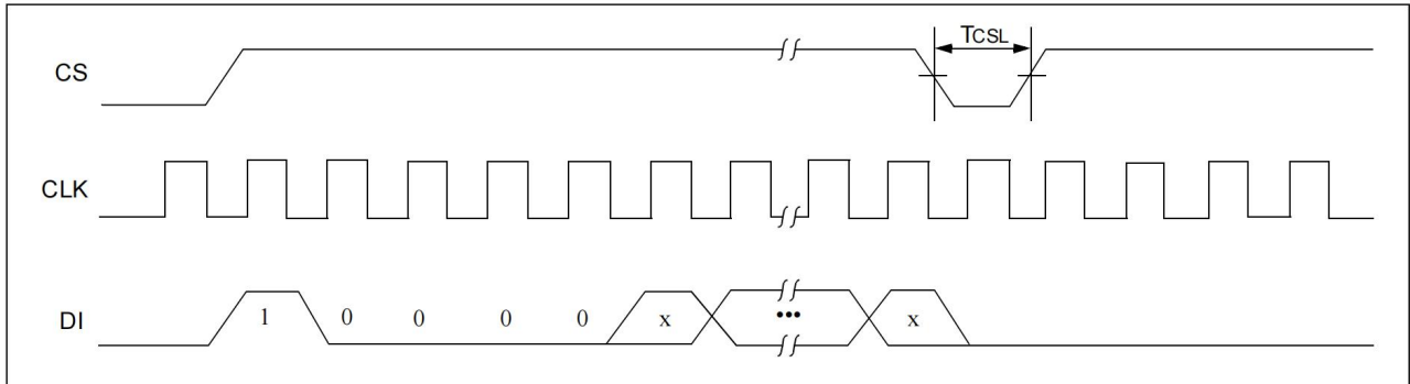
FIGURE 2-5: EWDS TIMING
