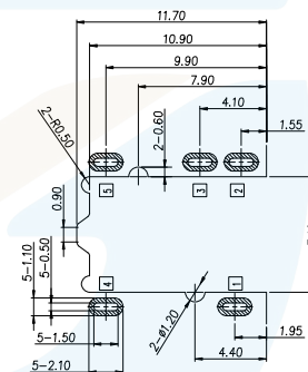
RECOMMENDED P.C.B LAYOUT TOP VIEW (TOLERANCE:±0.05)
