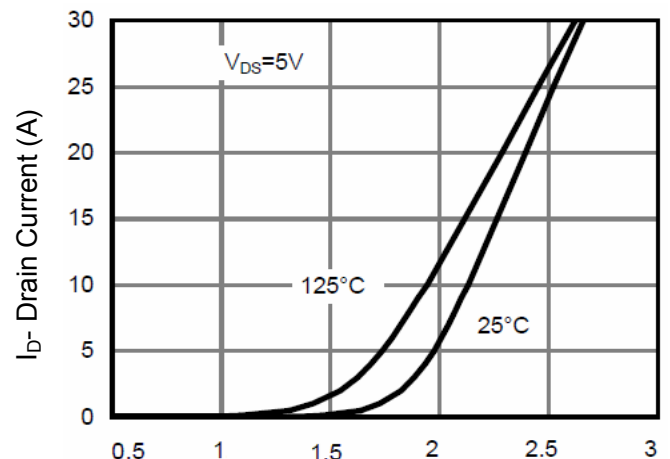
Figure 4 Transfer Characteristics
