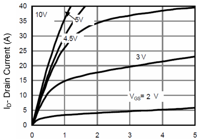
Figure 3 Output Characteristics
