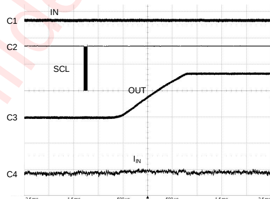
Figure 32 Inrush Current (ldsw_tr1/0=10)
