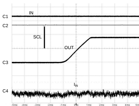
Figure 28 Inrush Current ( I_{dsw\_tr1/0}=10 )
