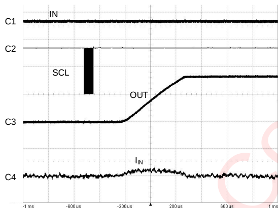
Figure 31 Inrush Current (ldsw_tr1/0=01)
