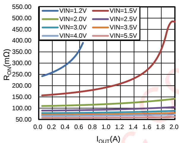
Figure 21 R_{ON} vs. I_{OUT} ( T_A=25^\circ C )
