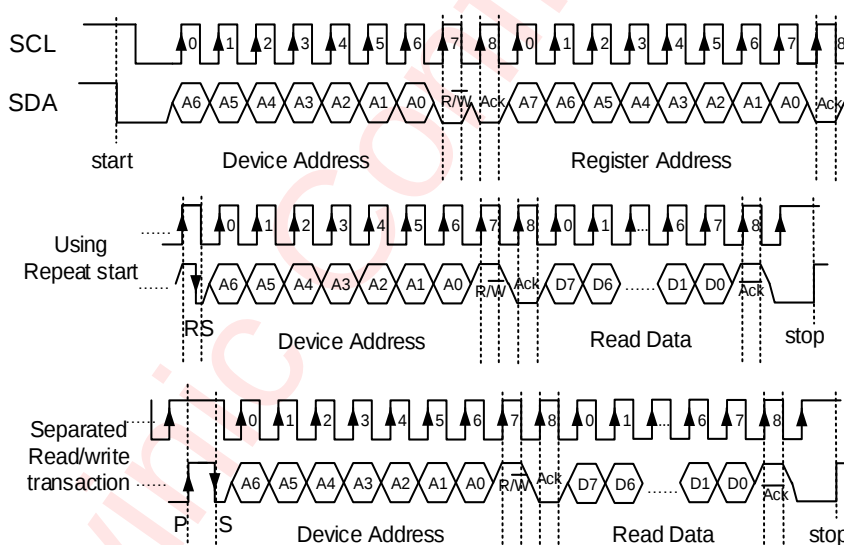
Figure 48 I²C Read Timing
