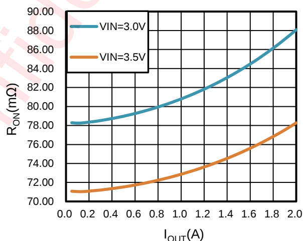
Figure 22 R_{ON} vs. I_{OUT} ( T_A=25^\circ C )
