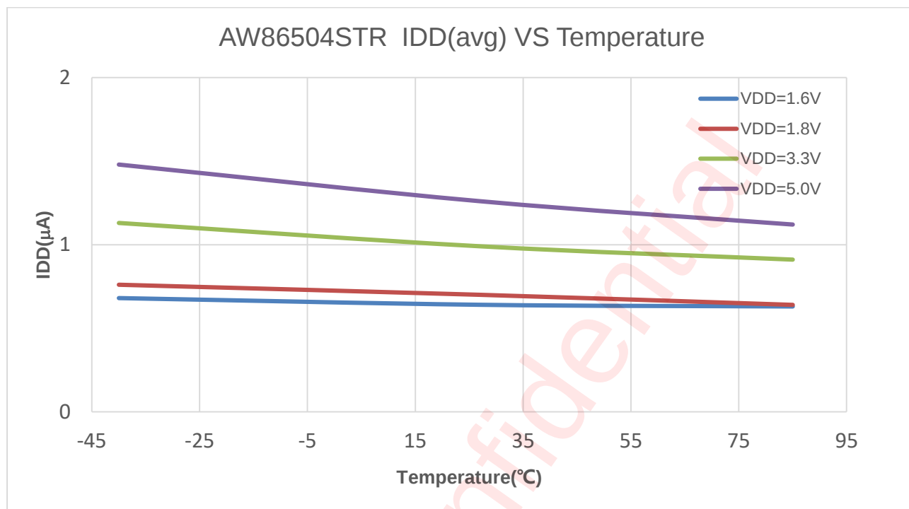
Ambient Temperature T_a [ ^{\circ}\text{C} ] I_{DD} vs. T_a
