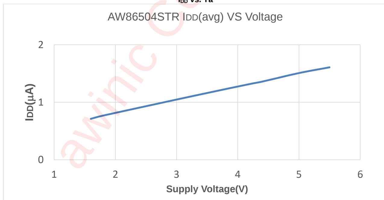
Average Supply Current vs. Supply Voltage( T_a=27^{\circ}\text{C} )
