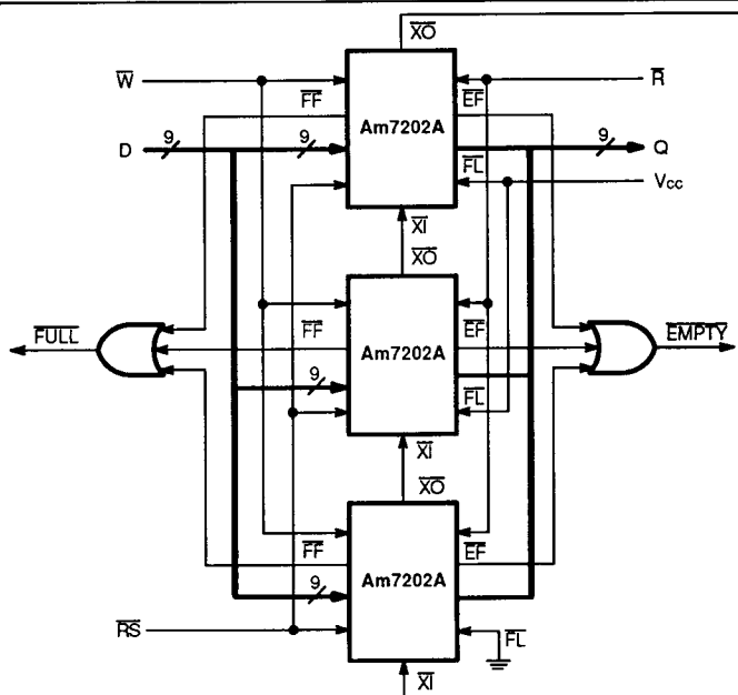
Figure 14. Depth-Expansion to Form 3,072x9 FIFO
