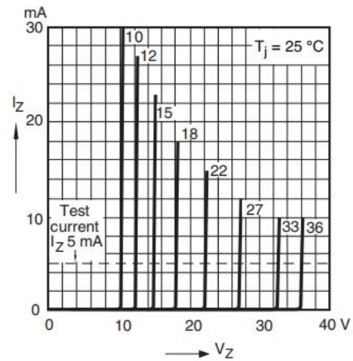
Fig.2-Zener Characteristic2
