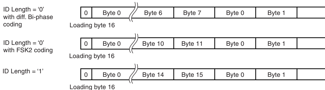
Figure 5-1. Examples of Different ID Length Settings
