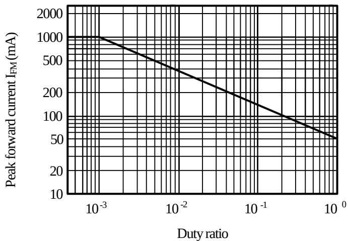
(Fig.7) Peak forward current vs. duty ratio
