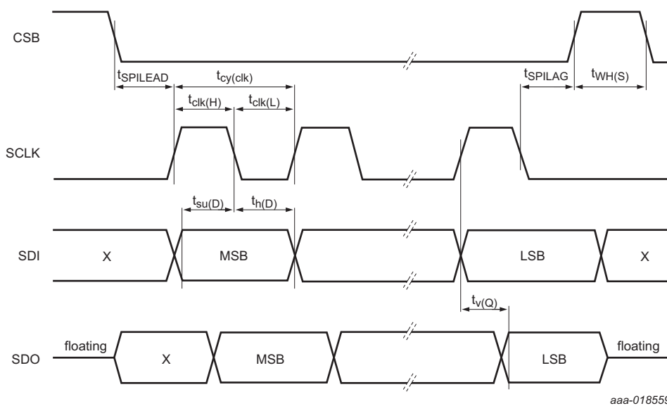
Fig 11. SPI timing diagram
