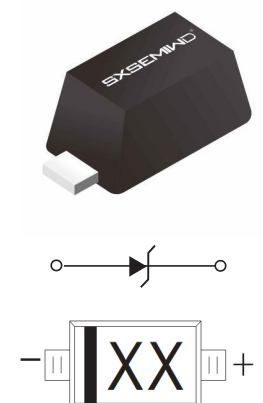
SOD-523
