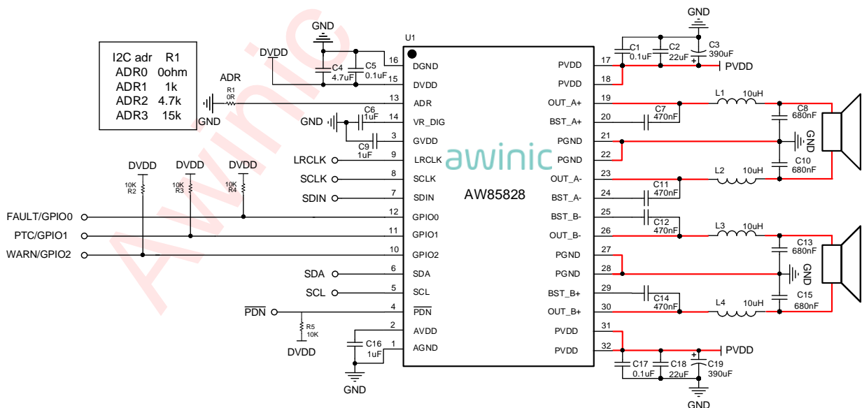
Figure 2 AW85828 BTL Application Circuit
