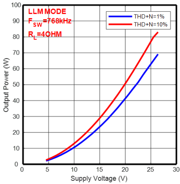
Output Power vs Supply Voltage -BTL
