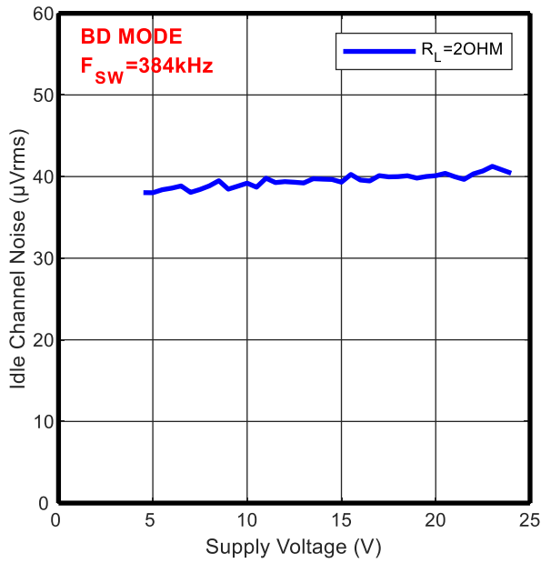
Idle Channel Noise vs Supply Voltage -PBTL
