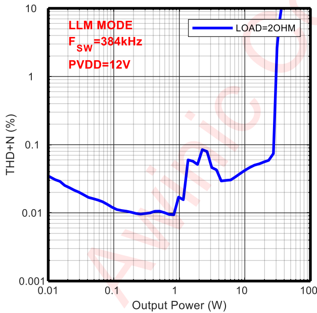
THD+N VS. OUTPUT POWER -PBTL
