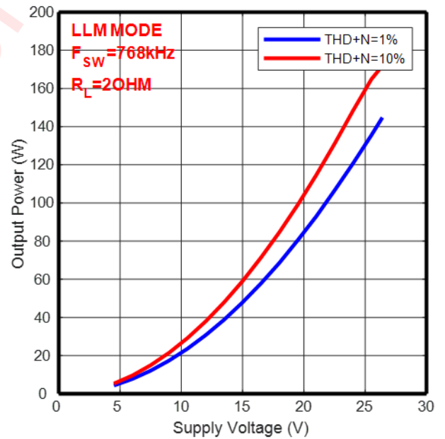
Output Power vs Supply Voltage -PBTL
