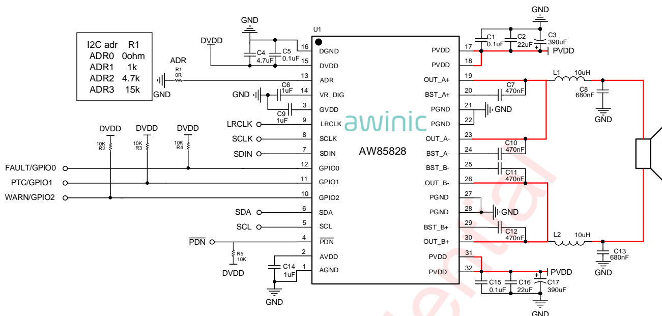
Figure 3 AW85828 PBTl Application Circuit
