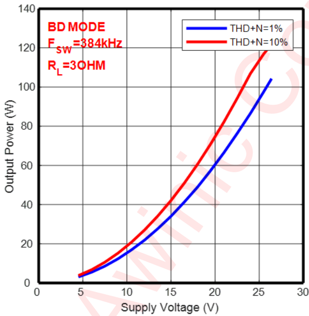
Output Power vs Supply Voltage -PBTL
