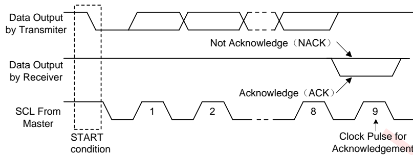
Figure 17 I 2 C ACK Timing
