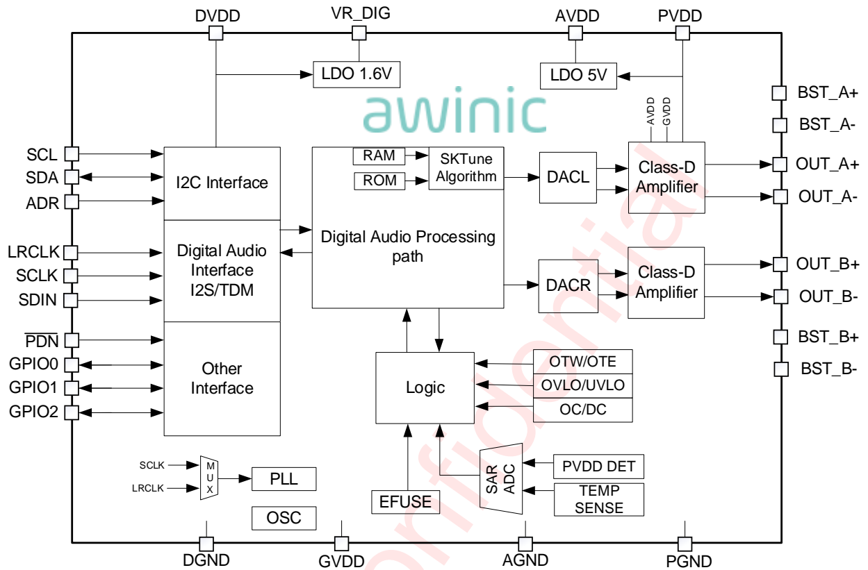
Figure 1 AW85828 Functional Diagram
