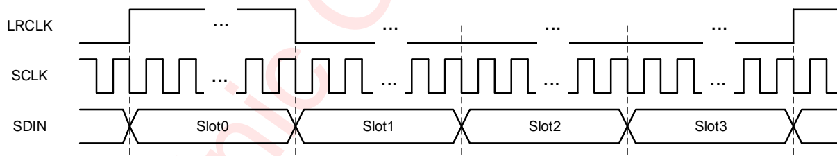
Figure 11 TDM Timing
