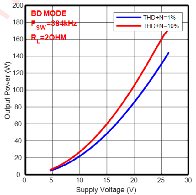
Output Power vs Supply Voltage -PBTL
